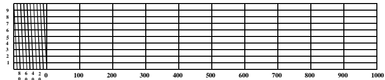
Figure 1 - Basic diagonal scale
