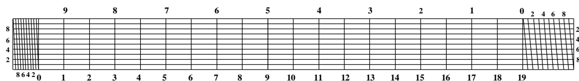
Figure 5 - Correct drawing of double diagonal scale on most Gunter rules
